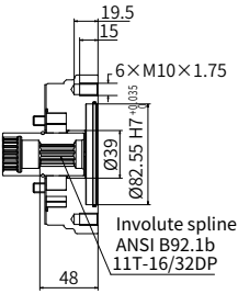
"A2" type through drive
