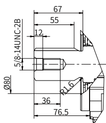
“C9” type spline shaft
