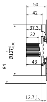
"C5" type spline shaft DIN 5480 W35×2×16×9g
