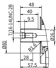
“C6” type spline shaft
