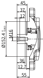
“D4” type spline shaft DIN 5480 W40×2×18×9g
