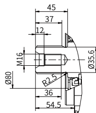
“CB” type spline shaft
