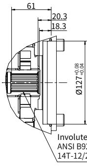
“C2” type through drive
