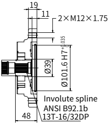
"B1" type through drive
