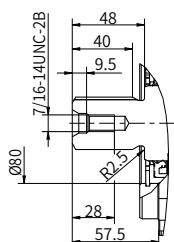
“C7” type spline shaft
