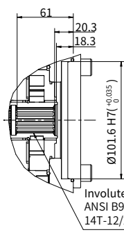
“B4” type through drive
