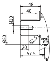
“C8” type spline shaft
