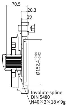
"D4" type through drive
