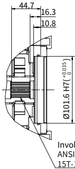
“B3” type through drive
