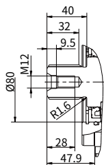
“CA” type spline shaft
