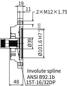
"B3" type through drive
