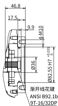
“A1”型通轴驱动
