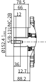
“D3” 型花键轴 ANSI B92.1b 2 in 15T 8/16 DP
