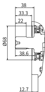
“C1” 型花键轴
