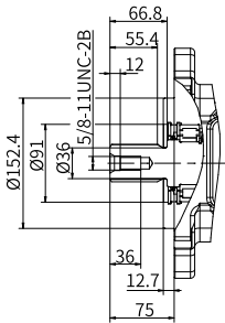
“D1” 型花键轴 ANSI B92.1b 1 3/4 in 13T 8/16 DP
