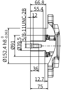
“D2” 型花键轴 ANSI B92.1b 1 3/4 in 27T 16/32 DP
