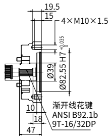
“A1” 型通轴驱动
